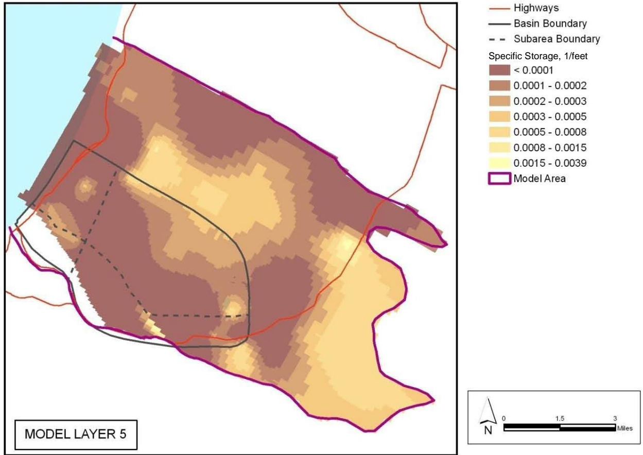
Figure 17. Model Calibrated Storage Coefficient for Model Layer 5 (Deep Aquifer)
